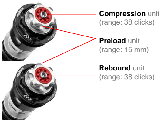
F25R-X cartridge fork kit Quad-valve asymmetric system
