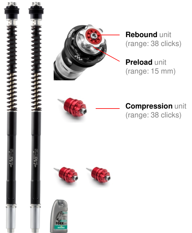
F25R fork kit
